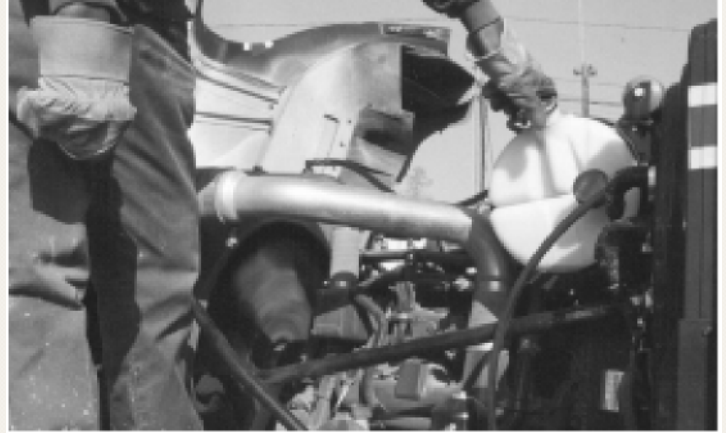
Figure 5-2: The CDP should check coolant levels during the pre-trip inspection. Never open the radiator cap when the engine is hot.
